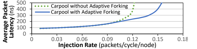
Figure 10: Effect of adaptive forking on average packet latency, for MedMC-MedHS .
